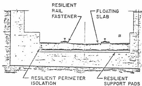
Figure 1. Cross section of continuous floating-slab design.
