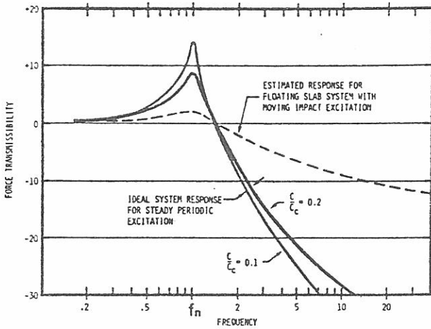
Figure 7. Force transmissibility response for single-degree-of-freedom vibration-isolation system.
