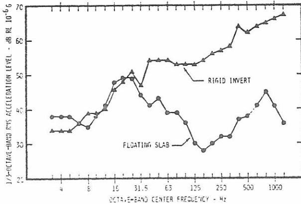
Figure 4. Subway-structure vibration levels with two-car Metro train passing at 64 km/h (40 mph).
