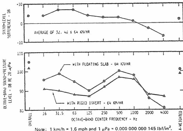
Figure 6. Average wayside noise level in subway with two-car Metro trains passing.
