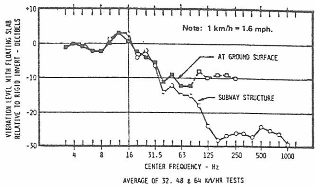
Figure 8. Insertion-loss performance of continuous floating-slab track bed as measured on surface and subway structure with two-car trains.
