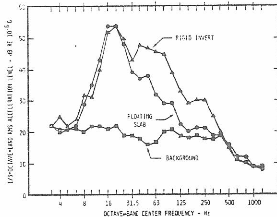
Figure 5. Ground-surface vibration levels with two-car Metro train passing at 64 km/h (40 mph).
