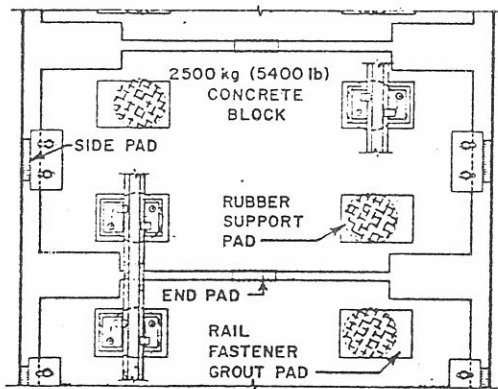
Figure 2. Plan view of discontinuous floating-slab design.
